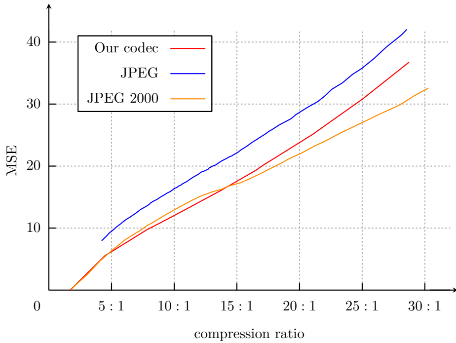
Figure 6.1: Comparison between our image compression codec, JPEG and JPEG 2000 for the grey scale version of the Peppers image. We consistently outperform the JPEG standard. For certain compression ratios between 5 : 1 and 15 : 1 we even outperform the JPEG 2000 codec. Also note that the JPEG format is always lossy. Even with parameters set to maximise the quality, loss of information occurs. Therefore, the JPEG curve cannot be extended to the left as far as for the other two codecs. The lowest compression ratio for our codec is achieved with a full mask. In that case the error is indeed 0 as we can simply store the original data and exploit the performance of the lossless PAQ compression.
