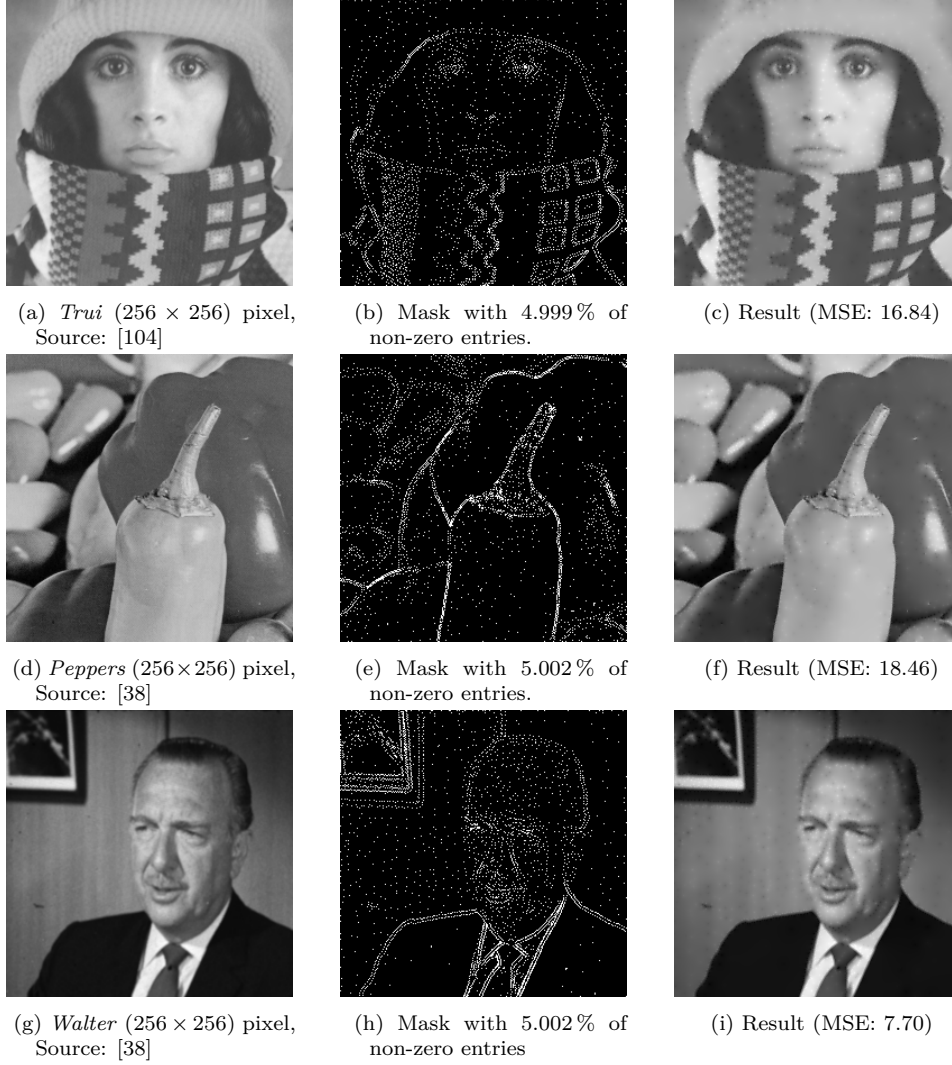
Figure 5.3: Results for three test images and a target density of 5%. All masks are sparse and yield a remarkable reconstruction quality. Note that the bright spots visible in the reconstruction are an artefact stemming from the fact that the Laplace operator is used. We set \lambda to 3.7 \times 10^{-3} for Trui , 3.26 \times 10^{-3} for Peppers , and 1.75 \times 10^{-3} for Walter . For these experiments the additional back projection is not performed.
