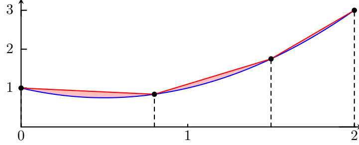
Figure 4.1: Visualisation of the free knot problem: We seek those positions of the the black dots along the blue curve such that the surface between the red and the blue curve becomes minimal (surface marked in pale red). Here, the blue curve represents the function x^2 - x + 1 and the red curve is the linear spline interpolating the function at the positions marked by the black dots.
