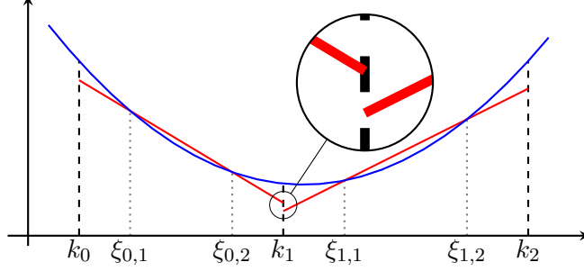
Figure 4.3: Approximation of f(x) = (x - \frac{3}{2})^2 + \frac{1}{2} (in blue) on the interval [\frac{4}{10}, \frac{13}{5}] with a piecewise linear spline (in red). On each interval [k_i, k_{i+1}] the line has been computed with Proposition 4.4. The corresponding optimal interpolation points given by this proposition are indicated as \xi_{i,1} and \xi_{i,2} . Note that the corresponding spline function has a discontinuity in the knot k_1 . Also, the function values of the spline do not coincide with the function values of f at the positions k_i .
