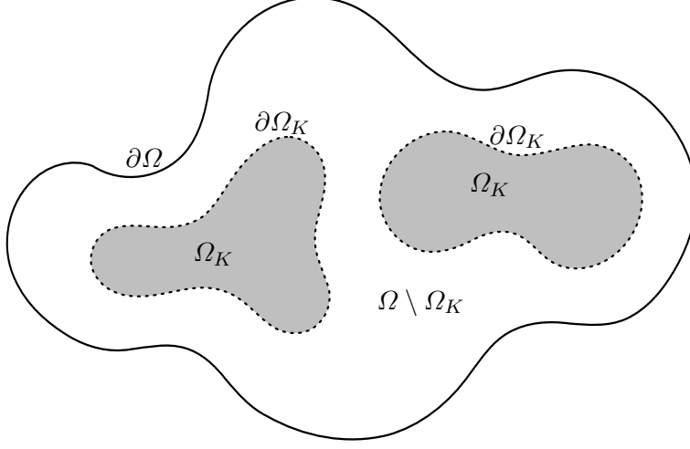
Figure 2.1: Example setup for a mixed boundary problem for PDE-based interpolation with the Laplacian. The set \Omega_K , marked in grey, denotes known data and is used to recover the missing information on \Omega \setminus \Omega_K by solving Eq. (2.1). Along the boundary \partial\Omega_K we assume Dirichlet boundary conditions whereas \partial\Omega \setminus \partial\Omega_K has Neumann conditions. Note that the set \Omega_K must have positive measure but it is not necessarily connected.
