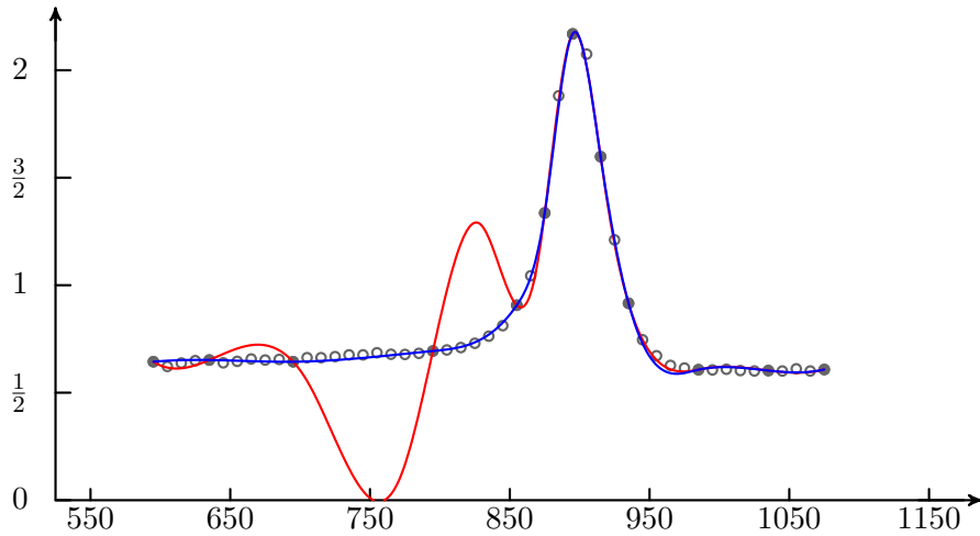
Figure 1.4: Interpolation of the popular titanium heat data (grey circles) [30] at the twelve locations marked by solid grey discs: The blue and red curve correspond to two cubic B-splines with different knot choices. Both splines interpolate the data at the same positions. The blue spline is considerably closer to the original data than the red spline.
