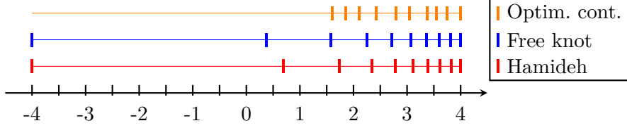
Figure 5.1: Mask distribution obtained by our frameworks for the function \exp(2x - 3) + x along [-4, 4] . Each rectangle represents the position of a mask point. The free knot method and the approach of Hamideh [63] fix the first and last knot at the endpoints of the considered interval. For the optimal control method all knots are free to move. For this experiment the additional back projection in the optimal control algorithm is not performed.
