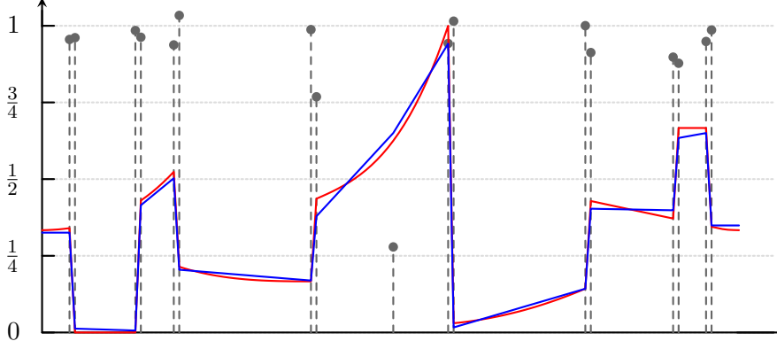
Figure 5.2: The original signal (red line), the reconstruction (blue line) as well as the used mask (grey dots). As expected, the mask is sparse (17 non-zero entries out of 128) and not binary-valued. Some knots even exceed the value 1. The mask point in the middle of the signal with the smallest value allows to better adapt to the curvature of the input signal by blending the diffusion result with the data. Also note that the mask entries neatly align with the discontinuities of the signal. This result is obtained with the parameter settings: \varepsilon = 10^{-9} , \mu = 1.0 , \lambda = 0.02 . For this experiment the additional back projection is always performed.
