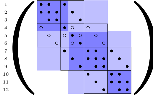
(b) The corresponding 12 \times 12 inpainting matrix. Black discs indicate non-zero entries. Black circles indicate entries that are 0 due to the choice of the mask values. All other entries are 0. The labels of the image have been placed next to the matrix rows for better orientation.
