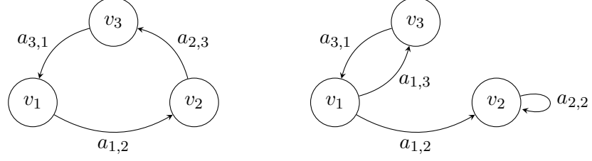
(a) A graph which is strongly connected. The corresponding adjacency matrix is given as A_1 in Eq. (2.7) (b) A graph which is not strongly connected. It is not possible to reach v_3 from v_2 . The corresponding adjacency matrix is given as A_2 in Eq. (2.7)
