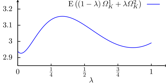
Figure 4.2: Evolution of the interpolation error with a linear spline for the function \exp(x) with mask points along the segment with endpoints \Omega_K^1 = \{-15, 10.65, 14.65, 15\} and \Omega_K^2 = \{-15, -1.2, 12.5, 15\} . It clearly depicts a non-convex behaviour. Note that the function values have been rescaled by a factor 10^{-6} for better readability.
