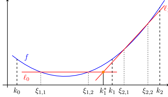
Figure 4.4: Visualisation of Hamideh's algorithm for updating the location of k_1 . The function f (marked in blue) represents our data function. The points k_0 , k_1 and k_2 denote the locations of the mask points from the previous iteration. On each interval [k_{i-1}, k_i] we compute the optimal interpolation points \xi_{i,1} and \xi_{i,2} using Proposition 4.4. These points yield two lines \ell_0 and \ell_1 (marked in red). The intersection point of these two lines (marked in orange) represents the next location of the mask point k_1^* . This strategy is repeated until a fixed-point is reached.
