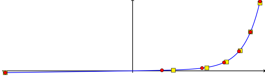
Figure 4.5: Distribution of 7 mask points along the interval [-4, 4] for our interpolation approach (red circles) and the method of Hamideh (yellow squares) for the function x \mapsto \exp(2x - 3) + x (marked in blue). Note that there are almost no points in flat regions, whereas there is a high density in regions with large curvature. The mask points of Hamideh do not necessarily lie on the function curve. Their positions corresponds to the coordinates yielded by Hamideh’s algorithm (well visible for the last mask point at the right).
