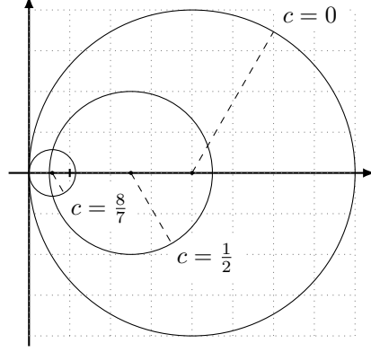
Figure 2.4: Visualisation of the Geršgorin discs for c = 0 , c = \frac{1}{2} and c = \frac{8}{7} with grid size h = 1 for some inner pixel ( |N(i)| = 4 ). The vertical tick is positioned at x = 1 and marks the position of the Geršgorin disc for c = 1 with radius 0. Note that the centre of the circles move from x = 4 to x = 1 when c changes from 0 to 1. At the same time the radius of the circles get smaller. For c varying from 1 to \frac{8}{7} the centres move from x = 1 to x = \frac{4}{7} and the radius increases from 0 to \frac{4}{7} .
